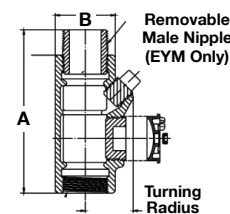
EYM 1-1/4" – 6"
