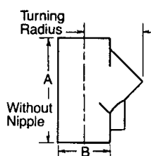
EYDM 1/2" — 1"
