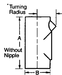
EYS 1-1/4" — 6"
