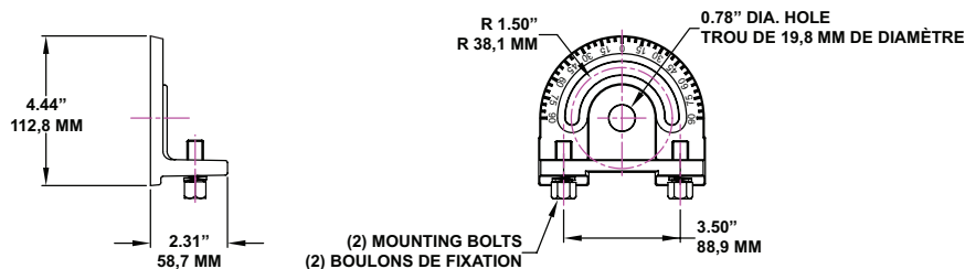
Figure 4: Crossarm Mounting Bracket (P/N: G-AM-8-CA) | Support de montage sur traverse (réf. : G-AM-8-CA)
